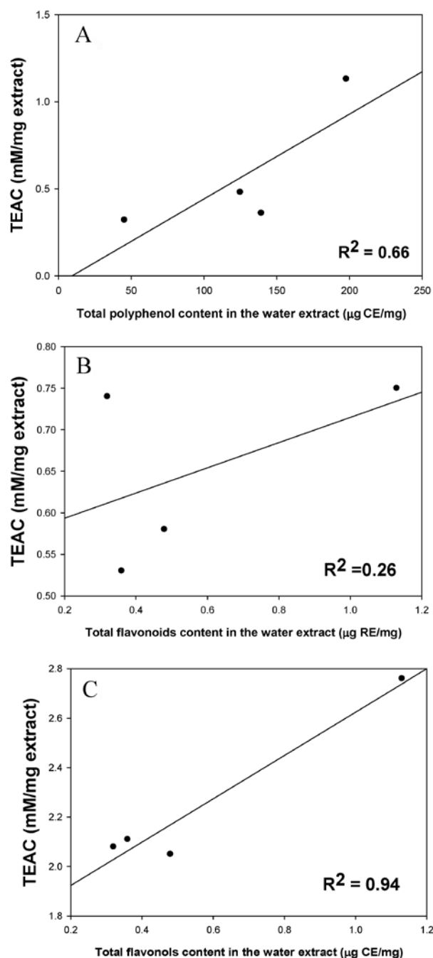
Figure 2. Correlation coefficients ( R^2 ) of TEAC and total polyphenol (A), flavonoid (B) and flavonol (C) contents in the aqueous extracts of the four Flemingia species.
