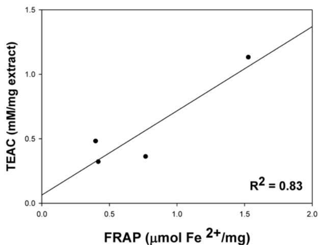
Figure 1. Correlation coefficients ( R^2 ) of TEAC and FRAP in the aqueous extracts of the four Flemingia species.
