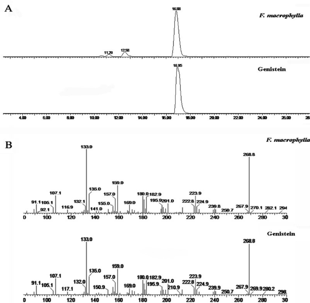
Figure 3. (A) High performance liquid chromatographic profile of genistein in WFM and genistein standard; (B) Daughter ion spectrum of major peaks in WFM ( R_t = 16.88 ) and genistein standard ( R_t = 16.95 ).
